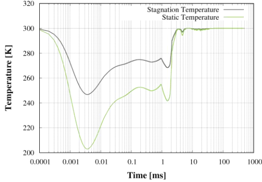
Fig. 4. Temperature dependency
