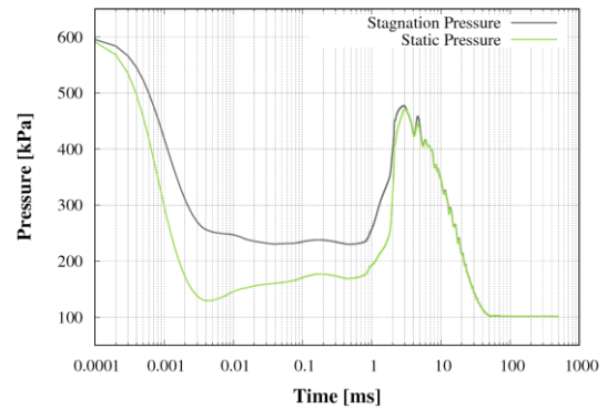
Fig. 3. Time dependency of inlet pressure
