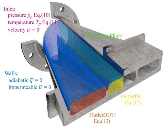
Fig. 2. Geometry model with numerical mesh visualized
