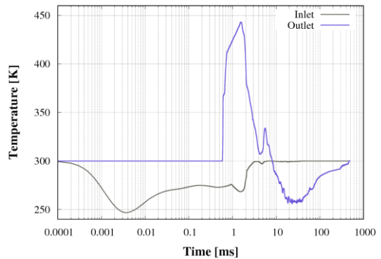
Fig. 7. Mean temperature values at inlet and outlet
