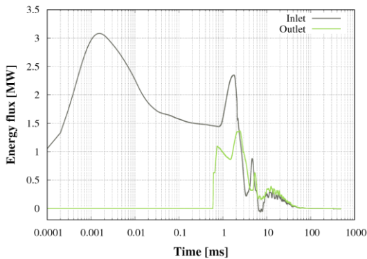
Fig. 9. Inlet and outlet energy fluxes
