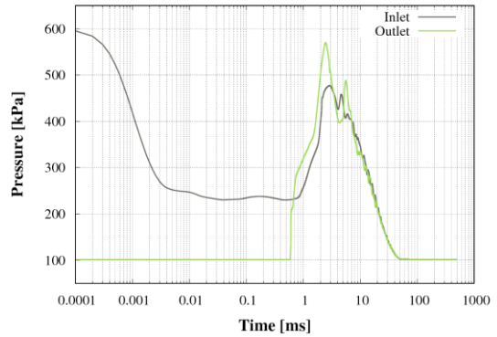
Fig. 6. Mean pressure values at inlet and outlet
