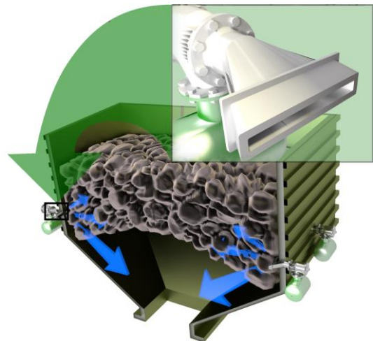
Fig. 1. Pneumatic pulsator system location on a silo walls with heatproof nozzle zoomed
