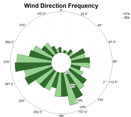
Fig. 4. Wind direction frequency – windrose
