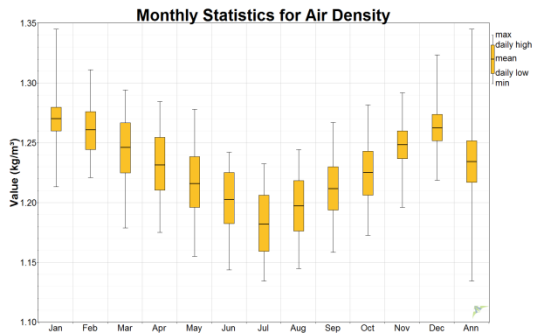
Fig. 7. Monthly average air density
