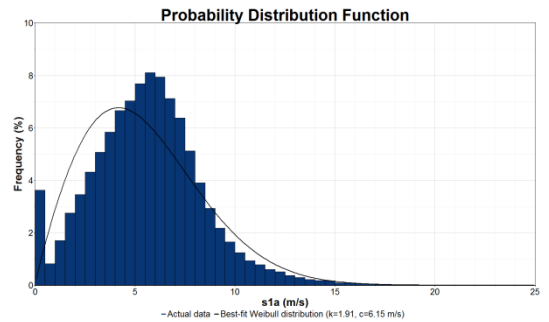
Fig. 3. Weibull's distribution for anemometer placed at the height of 80 meters
