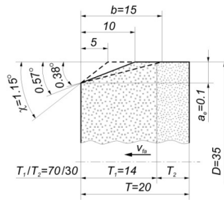
Fig. 2. The width b and the angle \chi of the grinding wheel conic chamfer shaped in experimental investigations
