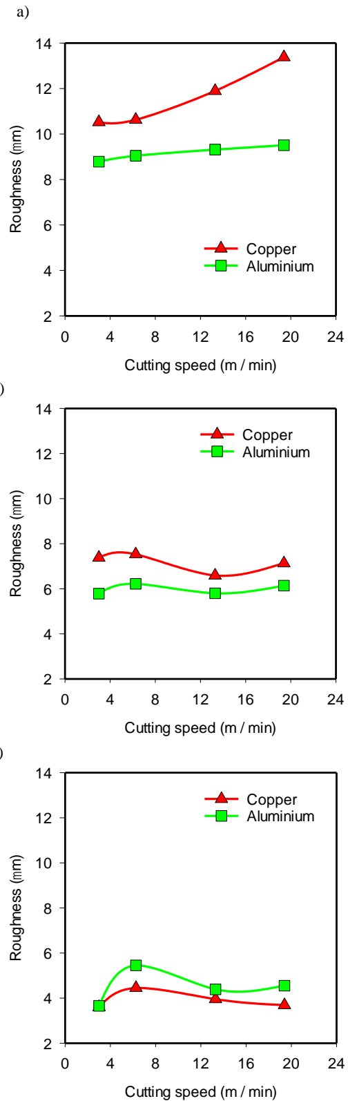
Fig. 8. Roughness of machined surfaces under different machining fluids and 1 mm depth of cut: (a) dry (b) kerosene and (c) soluble oil
