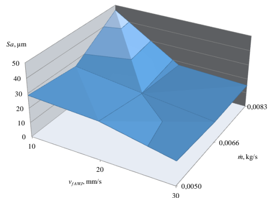
Fig. 12. Changes in the value of the parameter Sa of the surface after cutting sheet metal with a thickness of 10 mm depending on the variable feed speed of the v_{fAWJ} head and on the output of the abrasives m in the process of water-abrasive jet cutting
