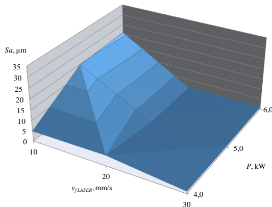
Fig. 9. Changes in the value of the Sa parameter of the surface after cutting 10 mm thick sheet steel depending on the variable power P and feed rate of the cutting head v_{fLASER} in the process of photon beam (laser) cutting
