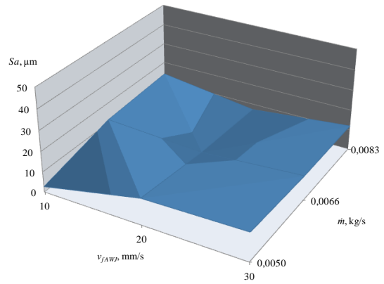
Fig. 11. Changes in the value of the parameter Sa of the surface after cutting sheet metal with a thickness of 8 mm depending on the variable feed speed of the v_{fAWJ} head and on the output of the abrasives m in the process of water-abrasive jet cutting
