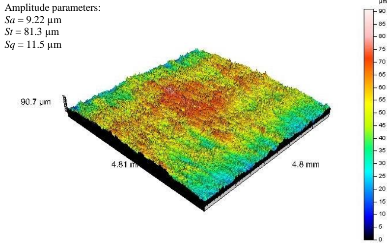
Fig. 5. Example of acquired surface microtopography after photon beam cutting
