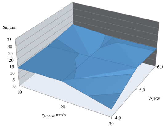
Fig. 7. Changes in the value of the Sa parameter of the surface after cutting 6 mm thick sheet steel depending on the variable power P and feed rate of the cutting head v_{fLASER} in the process of photon beam (laser) cutting
