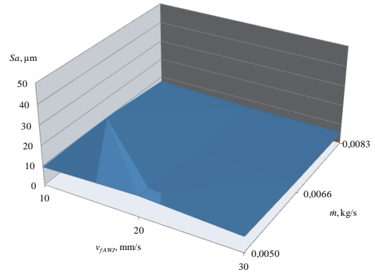
Fig. 10. Changes in the value of the parameter Sa of the surface after cutting sheet metal with a thickness of 6 mm depending on the variable feed speed of the v_{fAWJ} head and on the output of the abrasives m in the process of water-abrasive jet cutting
