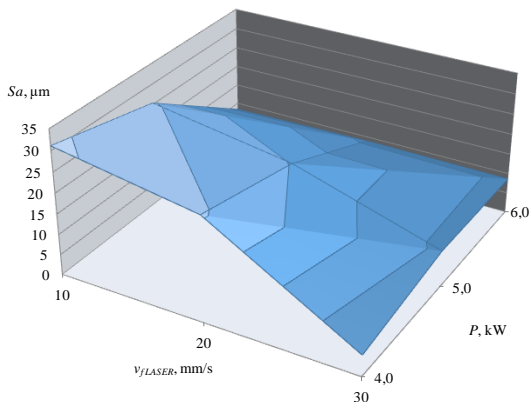
Fig. 8. Changes in the value of the parameter Sa of the surface after cutting 8 mm thick sheet metal depending on the variable power P and feed rate of the cutting head v_{fLASER} in the process of photon beam (laser) cutting
