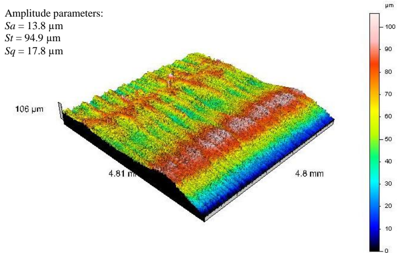
Fig. 6. Example of a acquired microtopography of a surface after abrasive water-jet cutting
