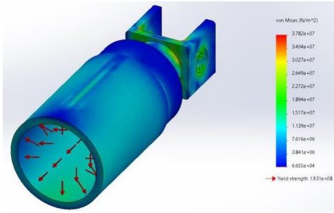
Fig. 4. Von Mises Stress in H1 with Al 5056
