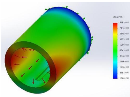
Fig. 13. Deformation in H2 with Al 7075
