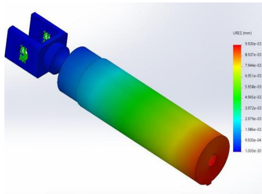
Fig. 9. Deformation in CR with Al 5056
