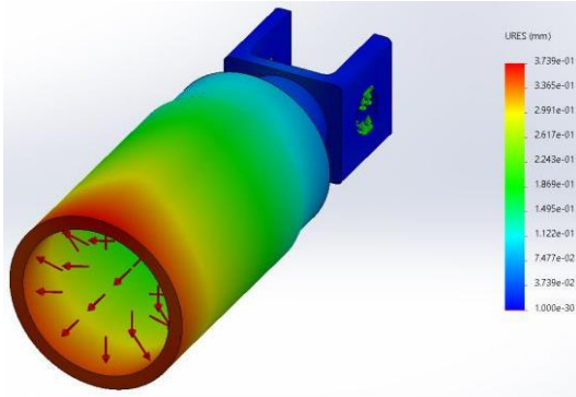
Fig. 11. Deformation in H1 with Al 7075
