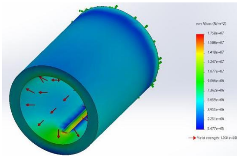
Fig. 6. Von Mises Stress in H2 with Al 5056
