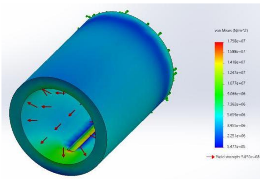
Fig. 12. Von Mises Stress in H2 with Al 7075
