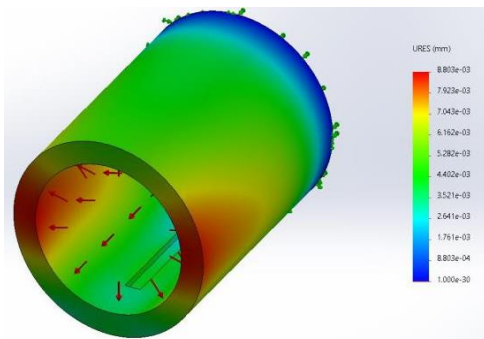
Fig. 7. Deformation in H2 with Al 5056
