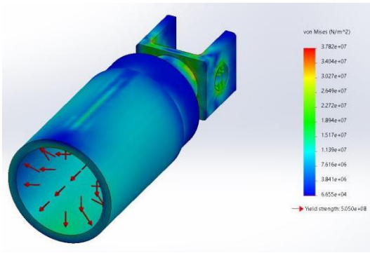
Fig. 10. Von Mises Stress in H1 made of Al 7075
