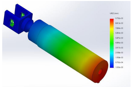
Fig. 15. Deformation in CR with Al 7075
