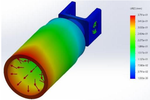
Fig. 5. Deformation in H1 with Al 5056
