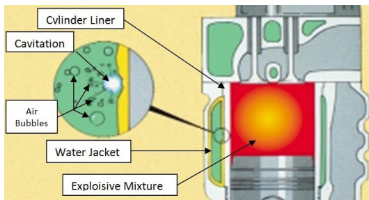
Fig. 6. Cavitation process
