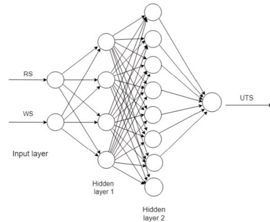
Fig. 3. Neural Network architecture used in this study
