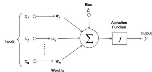
Fig. 2. Block diagram of Neural Network Architecture
