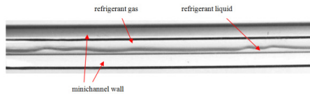
Fig. 10. Auxiliary description of the two-phase flow pattern image during the condensation of the HFE-7100 refrigerant in pipe minichannel with internal diameter d_i = 2 mm
