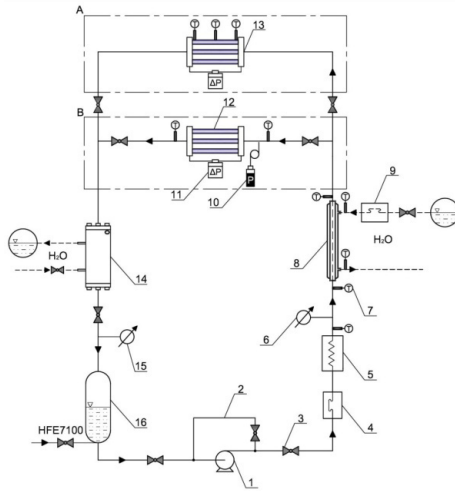
Fig. 2. Schematic of the test stand for thermal-flow and visualization of diabatic flow: A - Section for thermal and flow investigations, B - Section for experimental visualization of two-phase flow structures; 1 - ceramic pump, 2 - bypass for the flow control, 3 - valve, 4 - flowmeter for refrigerant, 5 - evaporator, 6 - manometer, 7 - K-type thermocouples, 8 - pre-heat exchanger "pipe in pipe" type, 9 - valve, 10 - flowmeter for cooling water, 11 - pressure sensor, 12 - differential pressure sensor, 14 - horizontal section for visualization, 15 - horizontal section of a heat-flow section 16 - valve, 17 - heat exchanger, 18 - vacuum pump, 19 - manometer, 20 - tank of liquid refrigerant HFE-7100
