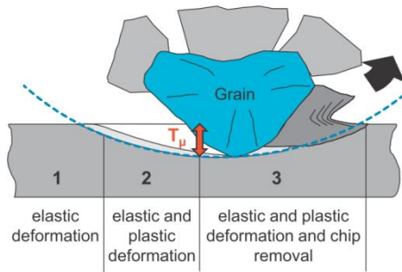
Fig. 3. Phases of chip formation in grinding [11]
