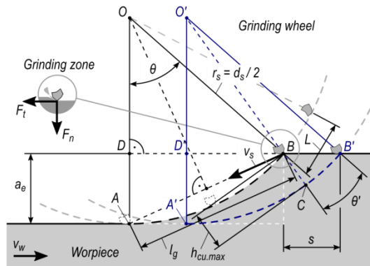
Fig. 1. The geometry of micro-scale surface material removal process by single grains
