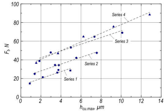
Fig. 6. Variability of the tangent component of the grinding force according to the machining conditions
